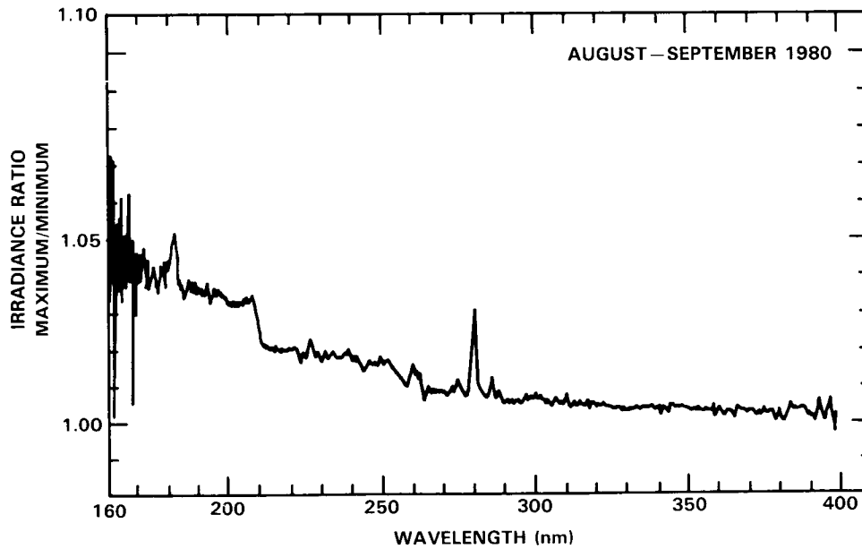
Figure 7-3. Variation in the solar irradiance over two 27 day rotation periods in November-December 1979 and August-September 1980. The ratio is of the maximum irradiance observed during the rotation to the mean of the preceding and following minima. Values are from the Nimbus 7 SBUV experiment (Heath et al. , 1984).
