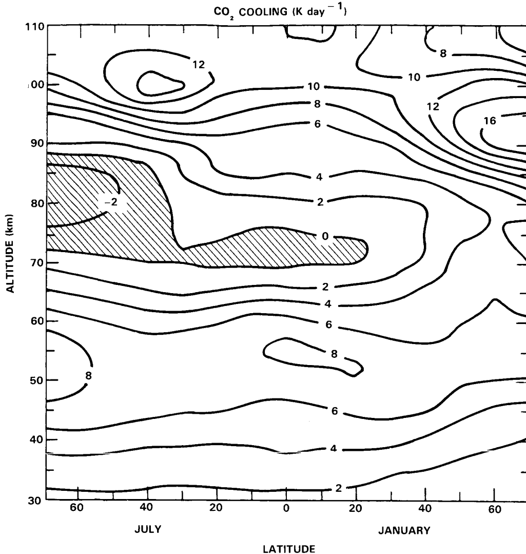
Figure 7-14. Longwave heating rate due to \text{CO}_2 in the upper stratosphere, mesosphere, and lower thermosphere for the January-July CIRA atmosphere (from Dickinson, 1984).
