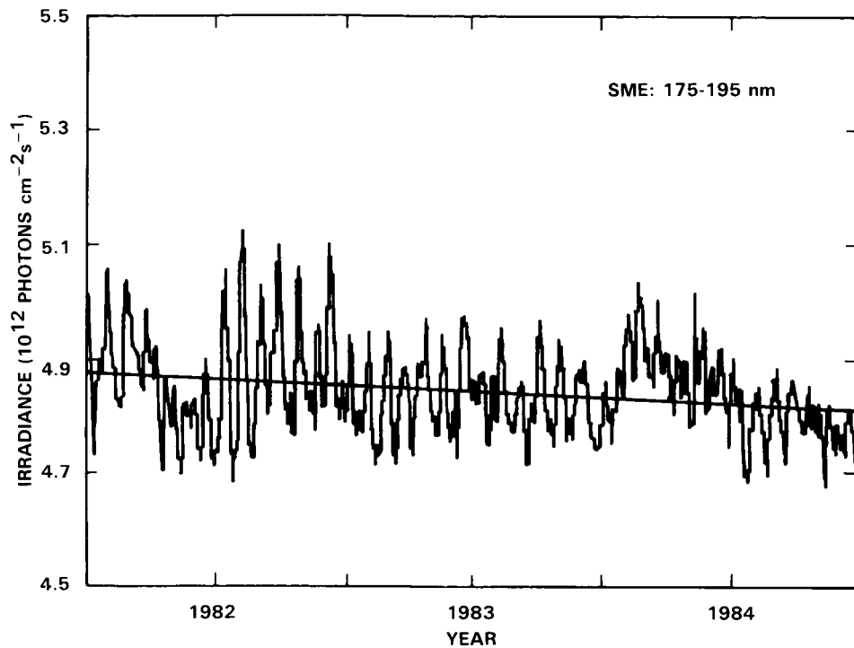
Figure 7-4. Variation in the 175-195 nm integrated irradiance over the period 1982 through 1984 observed from the Solar Mesosphere Explorer satellite. The straight line is a least squares fit to the measurements. (Data provided by G.J. Rottman.)
