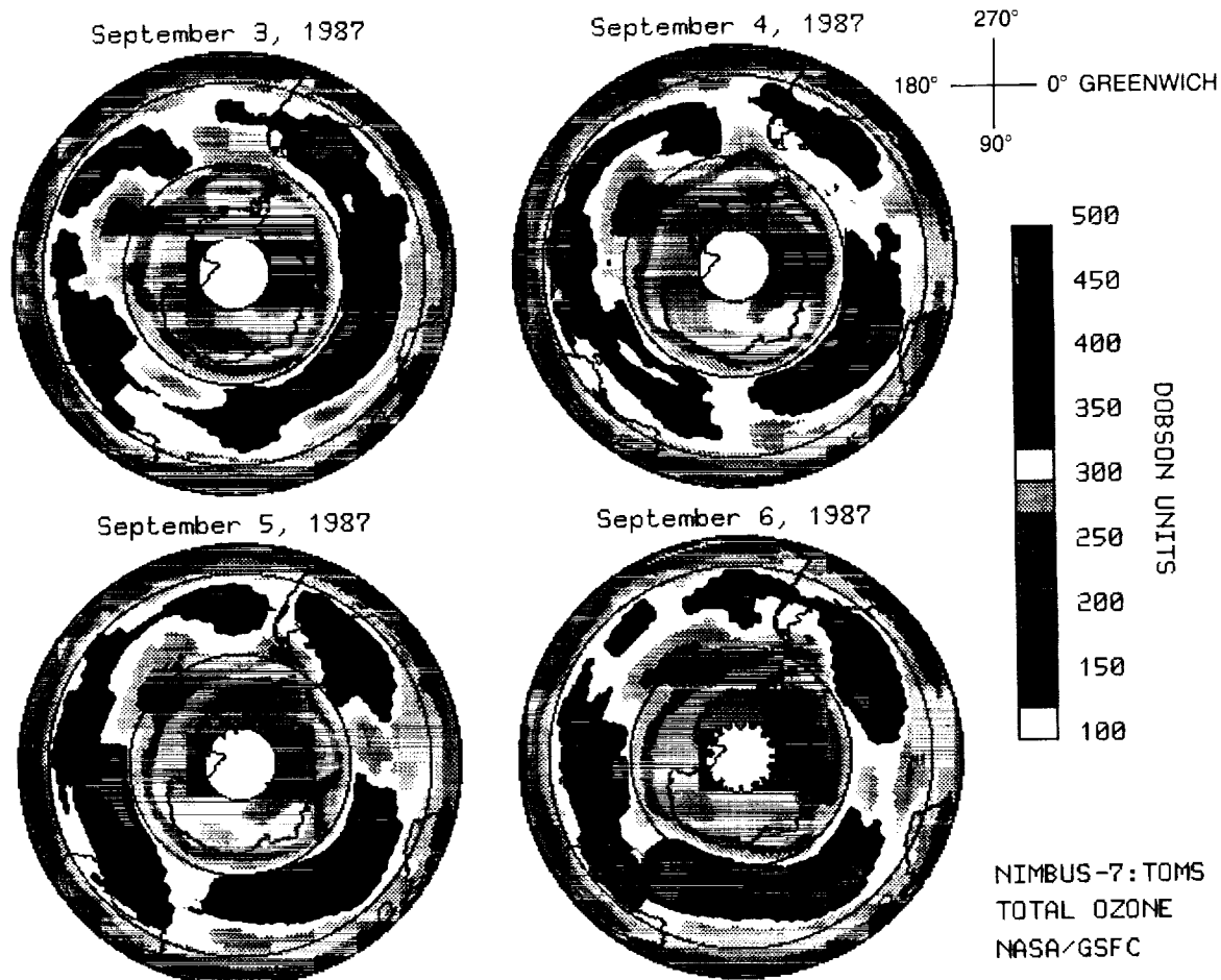
Figure 11.19. TOMS maps of total column ozone in the Southern Hemisphere for September 3–6, 1987. (Krueger, private communication.)
