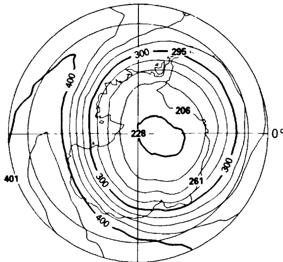
Figure 11.33. October 1983 maps of (a) temperature at 100 mb (hPa), (b) temperature at 30 mb (hPa), and (c) TOMS total ozone. Taken from Newman and Randel (1988).
