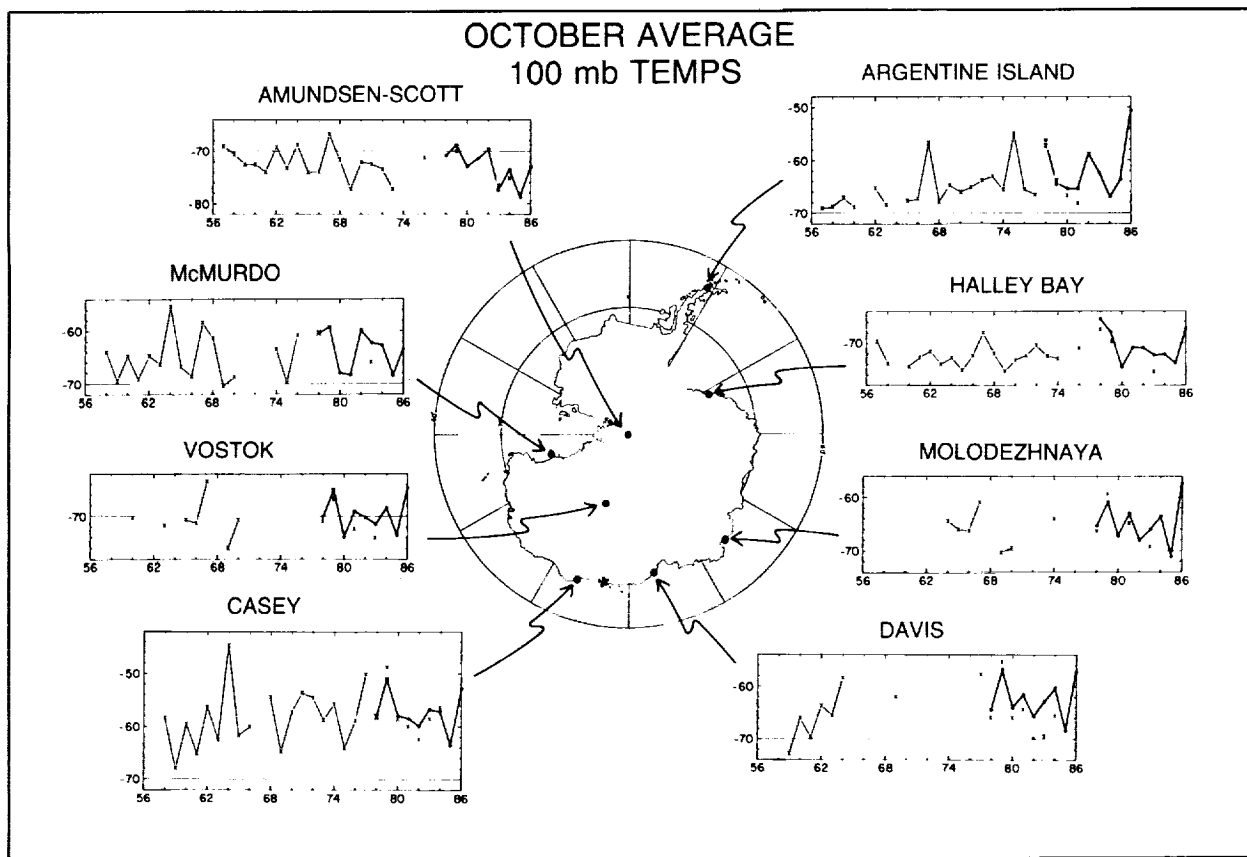
Figure 11.31. Time series of October mean 100 mb (100hPa) temperatures over eight Antarctic stations. Data from 1957–1984 are from rawinsonde observations (RAOB) and data from 1979–1986 are from NMC analyses.
