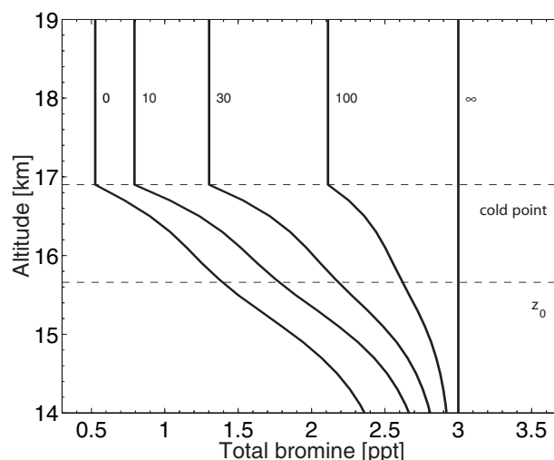
Figure 2-7. Calculated profile of total bromine from bromoform present as both product gas ( \text{Br}_y ) and source gas ( \text{CHBr}_3 ), defined as \text{Br}_y + 3 \times \text{CHBr}_3 , for different values of the lifetime of \text{Br}_y in days (numbers given in graph), based on a one-dimensional model of the tropical atmosphere. The calculations assume 1 ppt of \text{CHBr}_3 in the boundary layer and that no \text{Br}_y is detrained from convection (i.e., model assumes efficient uptake and removal of \text{Br}_y in clouds). Locations of the level of zero radiative heating and the cold point tropopause in the model are indicated. From Sinnhuber and Folkins (2006).
