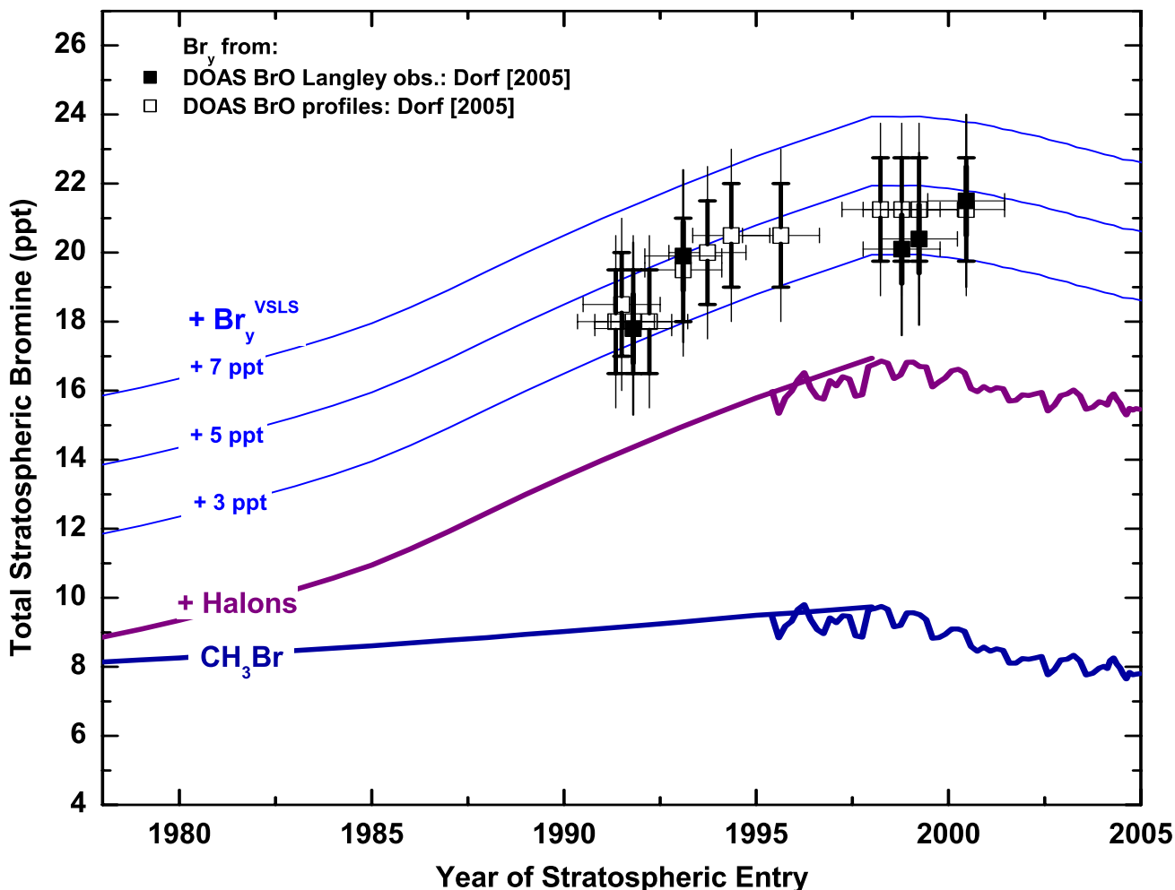
Figure 2-3. Trends (solid lines) of expected total inorganic stratospheric bromine ( Br_y ) due to measured tropospheric abundances of bromine from methyl bromide ( CH_3Br ; thick blue lines), the sum of CH_3Br plus halons (thick purple lines), and this sum together with assumed additional bromine (3, 5, and 7 ppt) derived from VLSL and/or inorganic tropospheric bromine sources (thin blue lines). This figure is an update of Figure 1-8 from the last Assessment (WMO, 2003). The smooth thick blue and purple lines prior to 1995 are based on a combination of Antarctic firn air reconstructions and ambient air measurements from a number of studies, adjusted to represent mean global abundances (references in WMO, 2003), and updated here with mean ambient air measurements (non-smooth blue and purple lines post-1995) from NOAA global monitoring stations (Montzka et al., 2003; updated). There may be small calibration differences between the different studies (see, for example, Fraser et al., 1999). The points (open and filled squares) are total inorganic bromine derived from stratospheric balloon measurements of BrO and photochemical modeling to account for BrO/ Br_y partitioning. The filled black squares are from the slopes of Langley plot BrO observations above balloon float altitude, while the open squares are lowermost stratospheric BrO measurements (Dorf, 2005, and Dorf et al., 2006a, and references therein; together with more recent data as described in Section 2.5.2.1). Bold/faint error bars correspond to the precision/accuracy of the estimates, respectively (Dorf, 2005). For stratospheric data, the date corresponds to the time when that air was last in the troposphere, i.e., sampling date minus mean age of air in the stratosphere. No correction has been made for gradients of CH_3Br in the troposphere (see text for discussion). Preindustrial levels of CH_3Br of 5.8 and 5.5 ppt have been inferred by Saltzman et al. (2004) from Antarctic ice cores and by Trudinger et al. (2004) from Antarctic firn air, respectively, whereas preindustrial levels of the halons have been reported to all be below detection limits in Arctic and Antarctic firn air by Reeves et al. (2005). Adapted from Dorf (2005); see also Dorf et al. (2006b).
