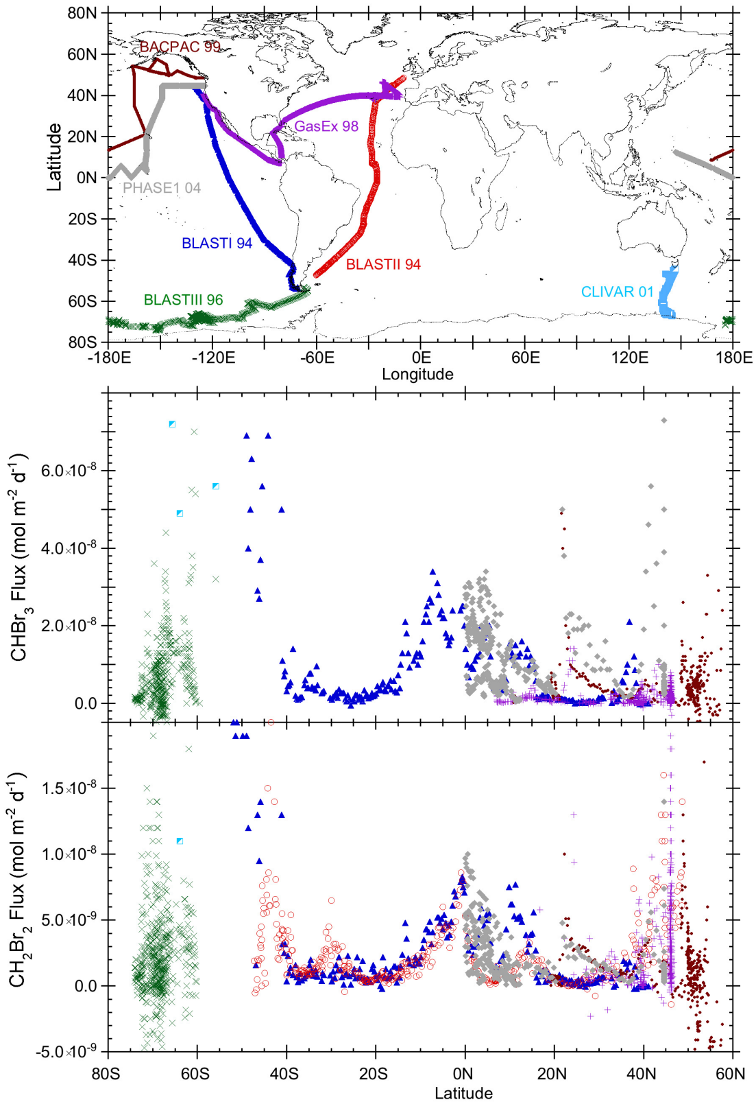
Figure 2-4. Plots of the oceanic fluxes of CHBr 3 and CH 2 Br 2 into the marine boundary layer based upon data from seven research cruises between 1994 and 2004 (Butler et al., 2006). Cruise data are color-coded to match those in the map. All measurements are on the same calibration scale.
